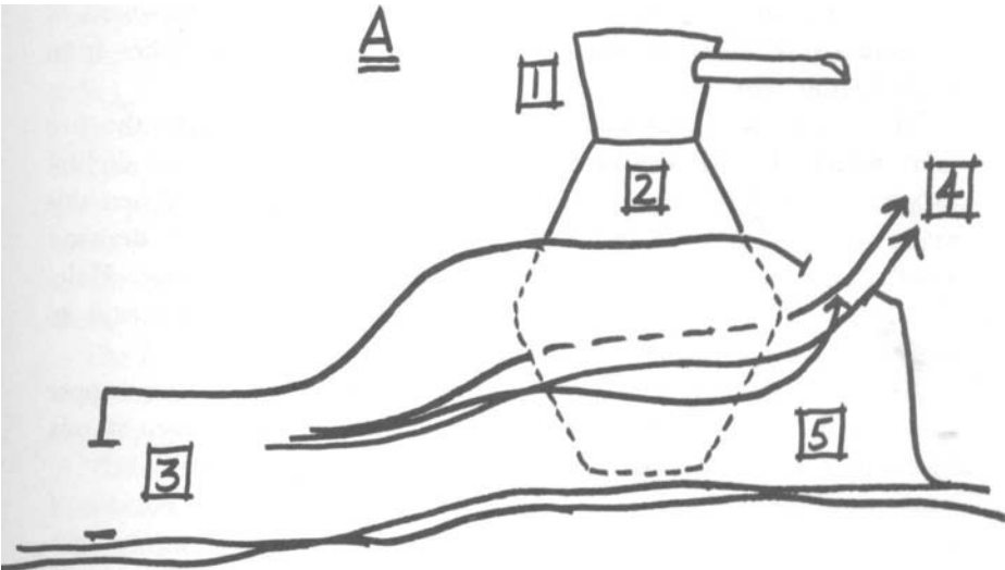
PLATE 266 Diagram A illustrates an interesting variation on furnace design which was once fairly popular. Called the "groundhog" or "hog" still, it was unique in that the still sat directly on the ground, and the furnace of mud, clay, and rocks was built up around it with the flue at the back. (1) is the cap, (2) the still, (3) the firebox. The heat was drawn to the flue (4) and circulated around the still in the space left between the furnace and the copper wall of the still. The arrows show the direction of heat. (5) is the back of the furnace—sometimes this was against a bank, and sometimes the furnace hole was dug directly into a bank. The surrounding earth, in the case of the latter design, was extremely effective insulation. When cleverly built, this furnace could also be much easier to hide than the stone furnace which sat right out in the open in most cases.
