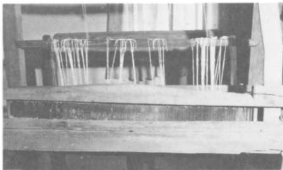
PLATE 257 Reed in place. Hed-dies in background.
