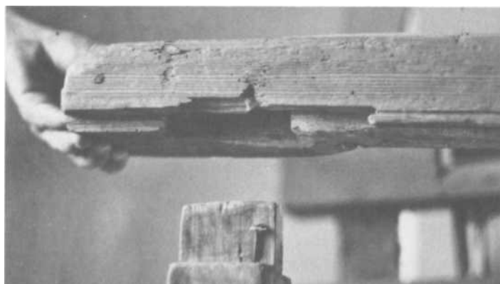
PLATE 275 Notches cut «n underside of beam fit top of loom frame
