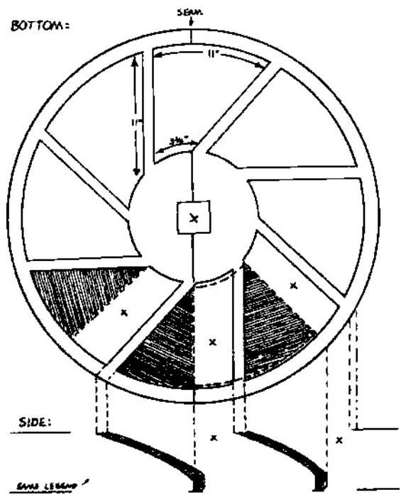
PLATE 153 The finished wheel from the bottom side.
