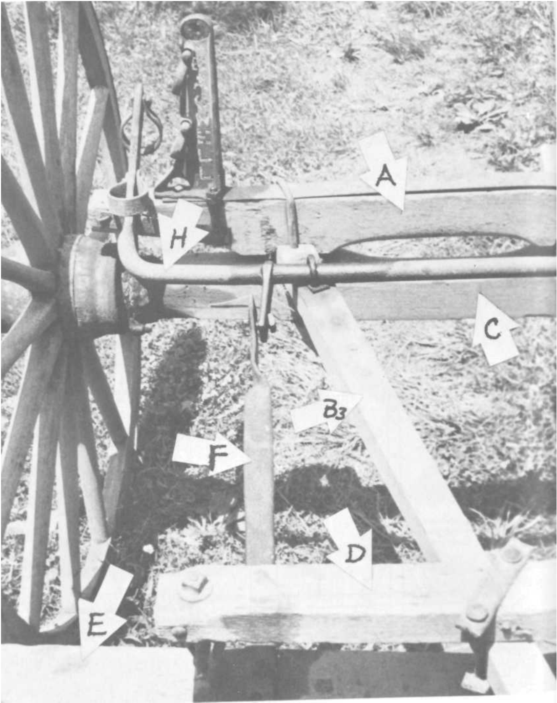
PLATE 120 Brake assembly. See diagram in Plate 121 .
