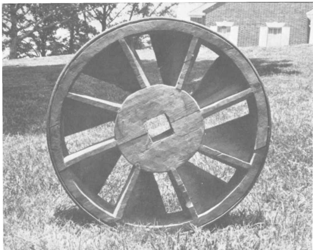
PLATE 151 The finished wheel from the top side.
