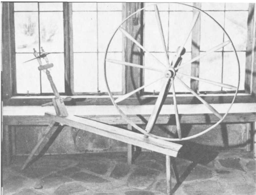
PLATE 227 Wheel #5 from the Hambidge Foundation.
