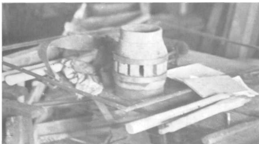
PLATE 79 John used a factory-turned hub for our wheel—ready for use except for the addition of the four bands. Traditionally the hubs would be turned on a foot-powered lathe, and the slots for the spokes cut with a sharp chisel. Here, the hub is ready for the last band to be added.
