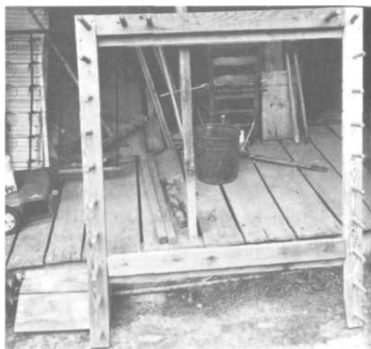
PLATE 294 Minnie Buchanan's hand-made warping frame—a little different, but it works on the same principle as Mrs. Brown's.
