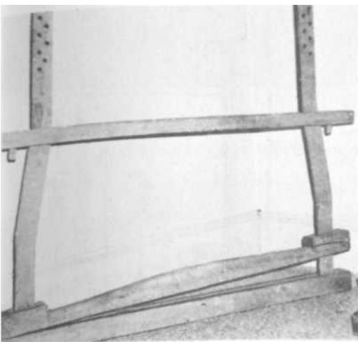
PLATE 256 Photo of beater frame without reed in place.
