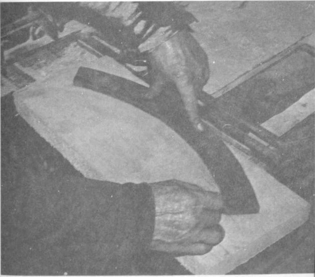
PLATES 90-93 A pattern is made for the wooden rim of the wheel (Plate 90), and the six felloes marked out on inch-and-a-half thick oak stock (Plate 91). Traditionally, these were cut out with a felloe saw (Plates 92—93 on p. 124).
