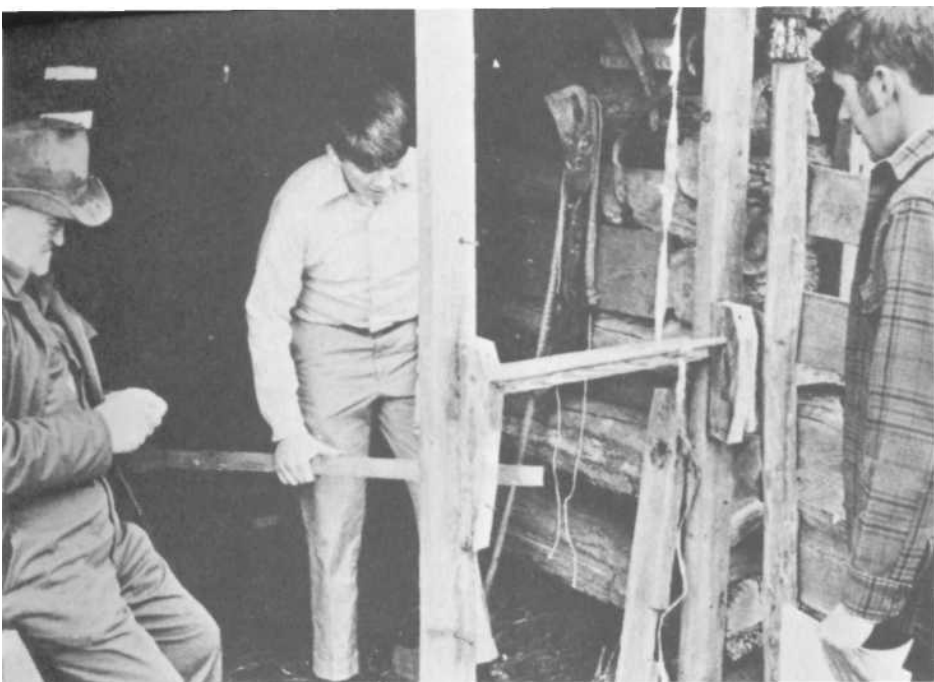
PLATE 168 The "H"-shaped frame for the lathe is two upright, seven-foot-long 2X4's and a horizontal beam; and two wooden brackets—a hole on the inside surface of each—for holding the stock to be turned.
