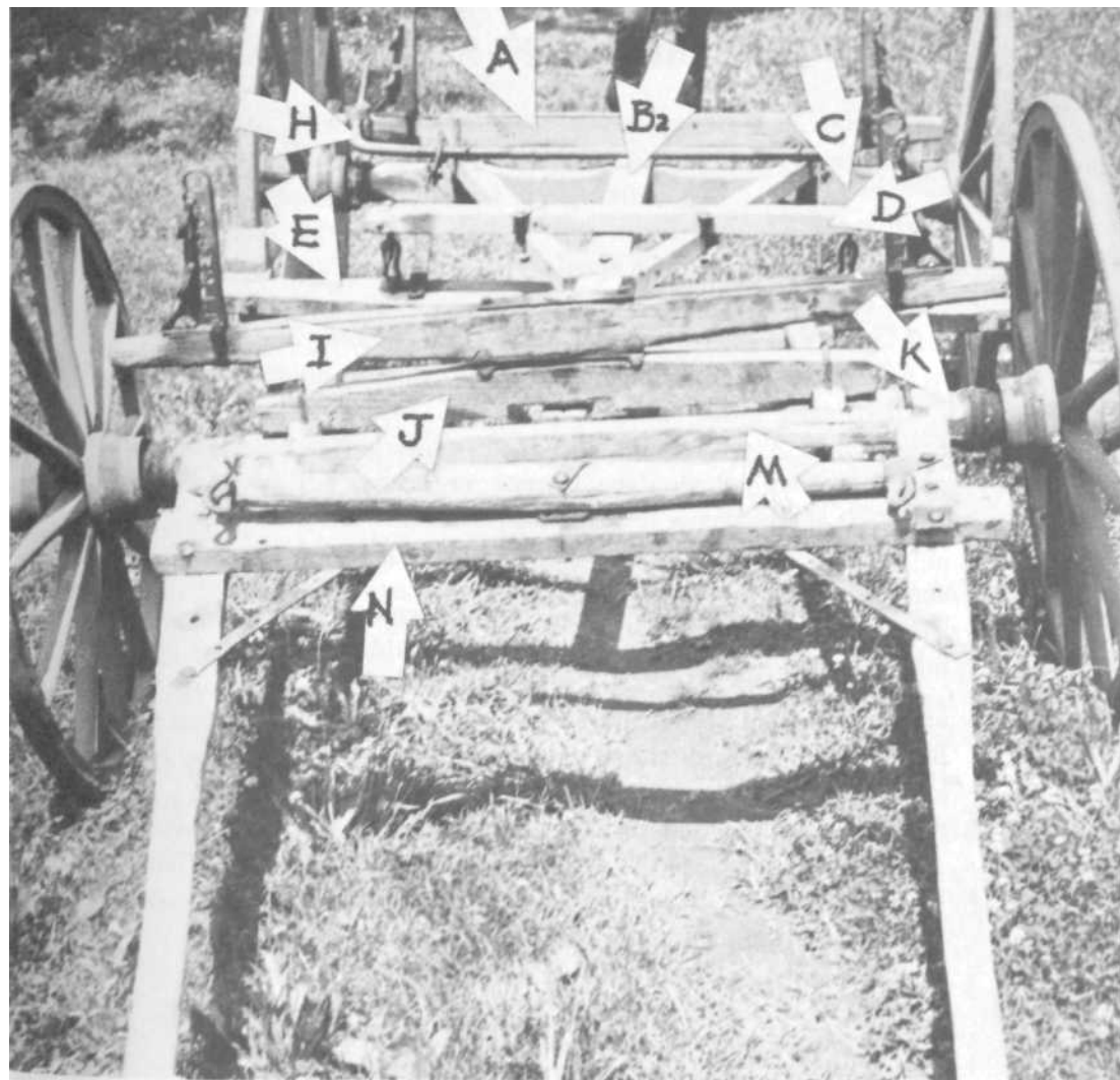
PLATE 125 The entire wagon seen from the front
