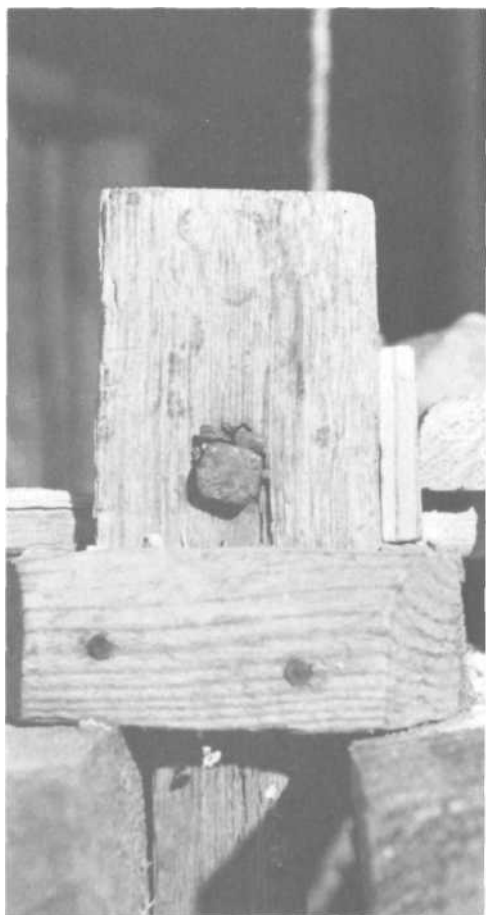
PLATE 181 Of special note are the two end pieces that hold the stock being turned. Rather than being mounted permanently on the vertical support beams, as on Minyard's lathe, these are cross-shaped pieces that slide back and forth between two horizontal beams (as shown here and in Plate 180 ) so that stock of varying lengths can be worked. The stock is held on either end by a metal spike driven through each cross-shaped end piece.
