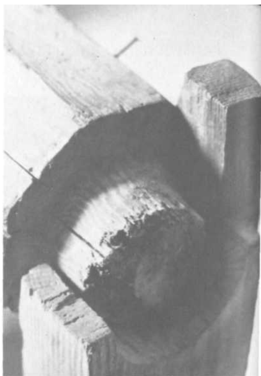
PLATES 270-271 Details of the two ends of the beam in place in the loom frame.
