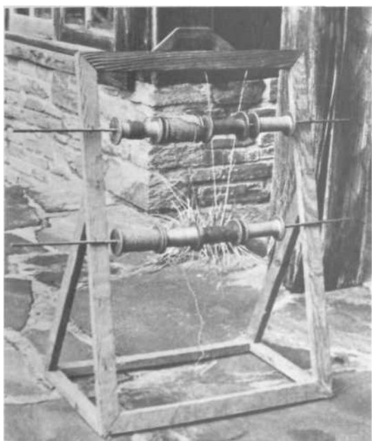
PLATE 247 Filled spools can be mounted on a SPOOL RACK. The number of spools set into the rack depends on the number of threads the weaver wishes to feed into the warper.
