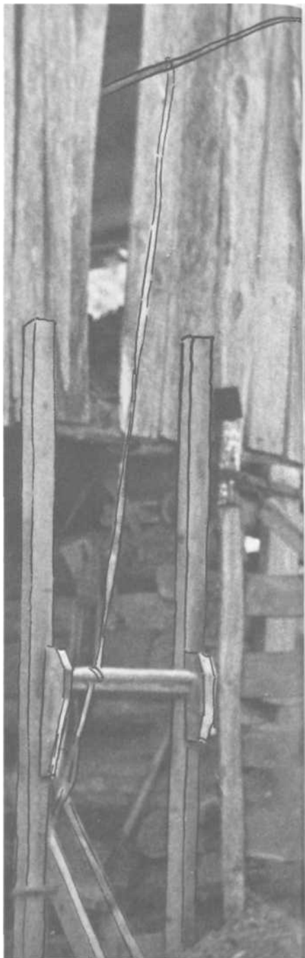
PLATE 176 Each time the pedal is depressed, the pole pulls the pedal back to the return position, spinning the stock in the opposite direction.
