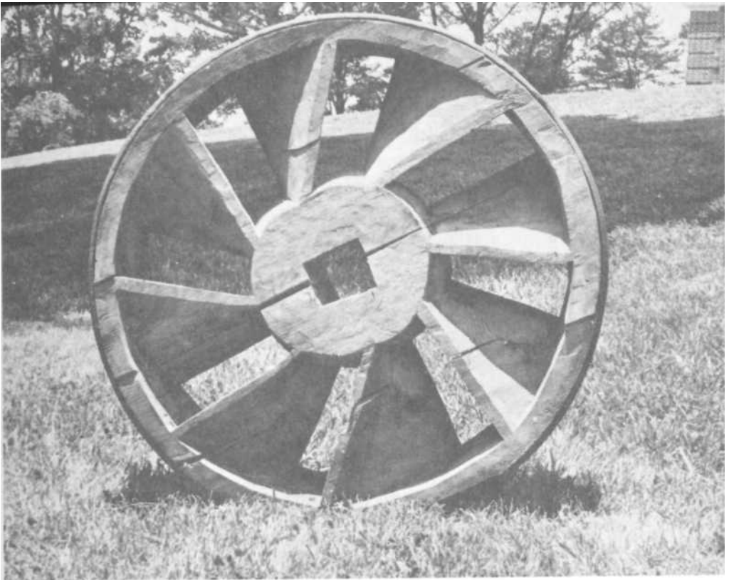
PLATE 153 The finished wheel from the bottom side.
