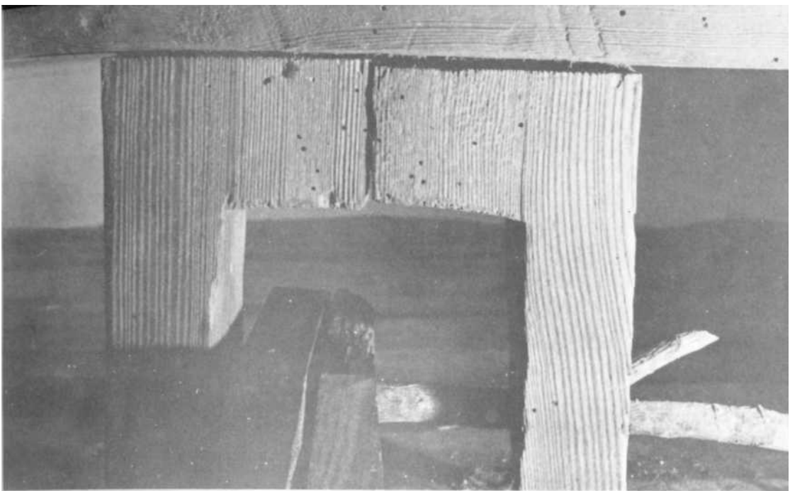
PLATE 277 Closeup of the piece that holds the ends of the treadles.
