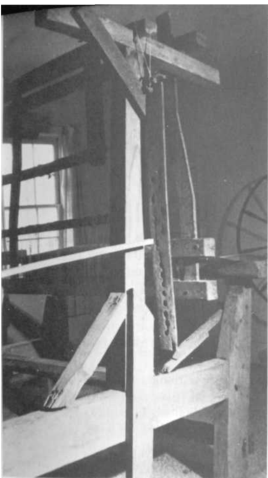
PLATE 286 The loom frame from its side.
