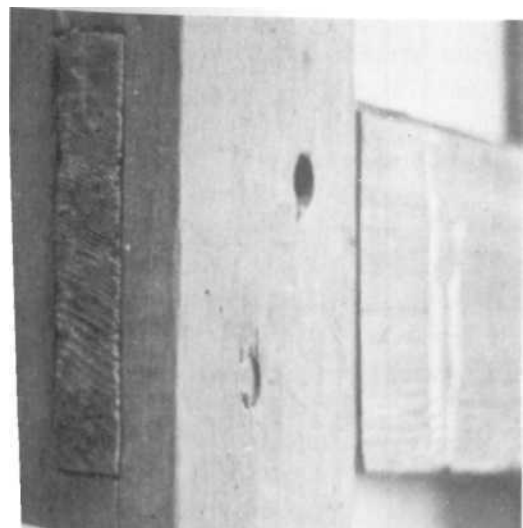
PLATE 288 Detail showing how side beam fits into loom leg. Note mortise and tenon joint with pees.
