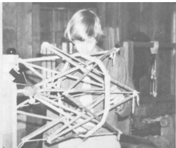
PLATE 245 The SWIFT was not widely used traditionally, but it does save work and is common today. The sliding wooden screw (arrow) clamps the expandable swift in position in either its expanded (shown here) or contracted position. A skein is slipped over a contracted swift, and then the swift is expanded.
