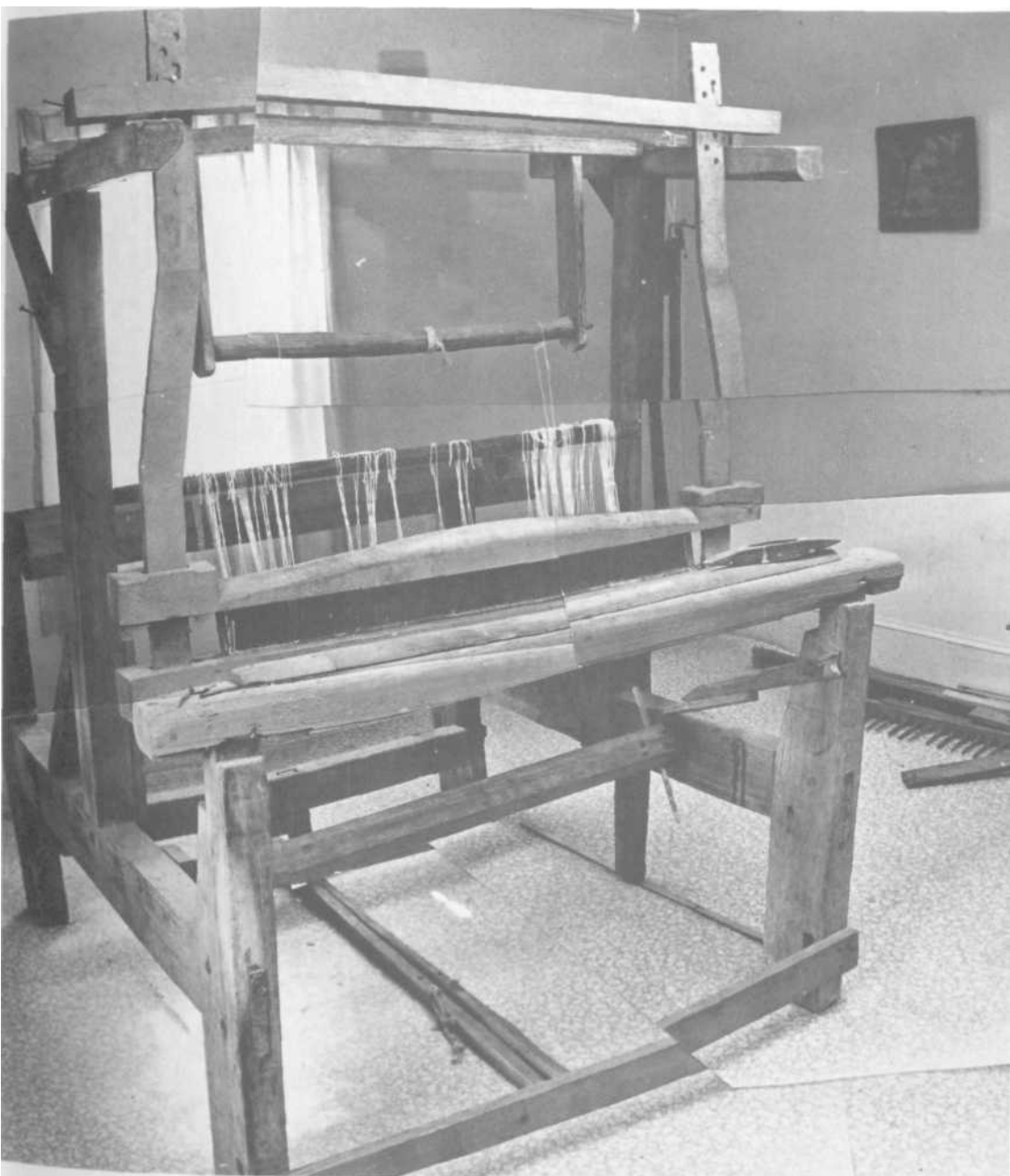
PLATE 254 This photograph shows the entire loom assembled. The room was so small that we couldn't photograph it assembled with our widest camera lens. So we had to try to lit several photos together. There is some distortion, but we hope you can ligurc it out. Details of the various pieces follow.
