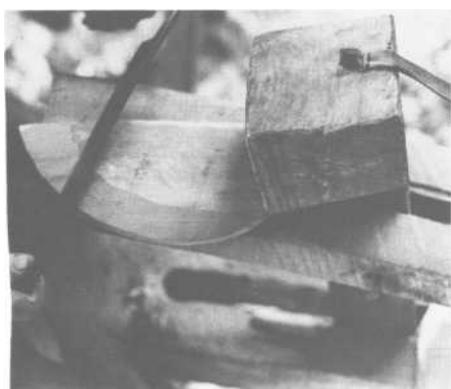
PLATE 364 Step 12: Begin to bevel the edges of the half-circles with a drawing knife.
