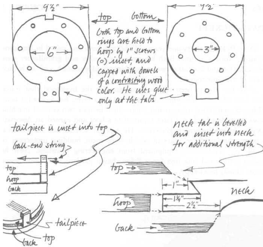
PLATE 121 The banjos that Leonard Glenn makes are similar in construction to those of both Tedra and Stanley (three wooden rings, a metal ring to hold the head, no neck extension, etc). There are several differences worth noting, however, as shown.
