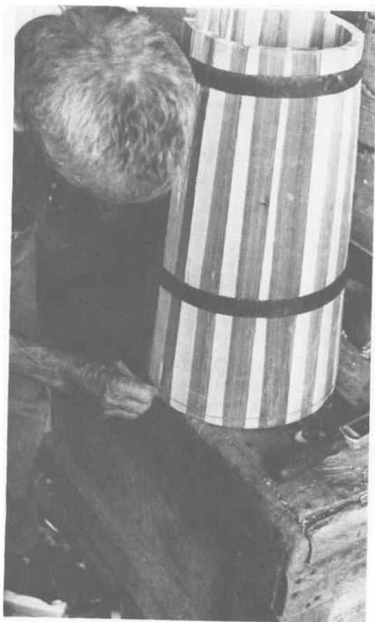
PLATE 371 Step 15: To measure for a permanent bottom hoop, take a string and measure the very bottom of the churn.
