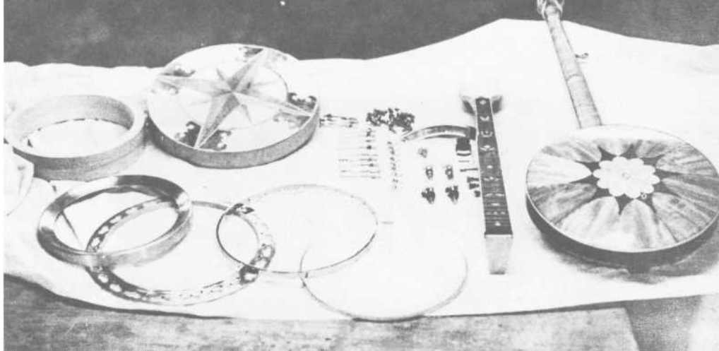
PLATE 150 The component parts of the most elaborate Sturgill banjo laid out. They include a fully inlaid resonator.
