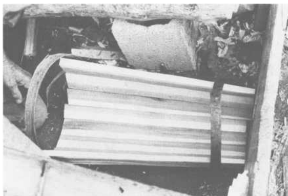
PLATE 344 The large hoop goes around the bottom (head) and the small one around the top. (Alex used a metal hoop for the top end and an old wooden hoop with a double knot fastening it at the bottom end.)
