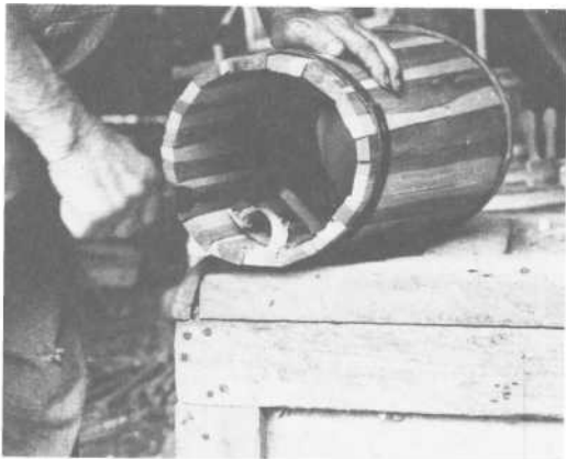
PLATE 351 Step 7: Using a round-shave, smooth (or dress) the inside of the churn. It is especially important to smooth the inside near the bottom end, where the head will be fitted.
