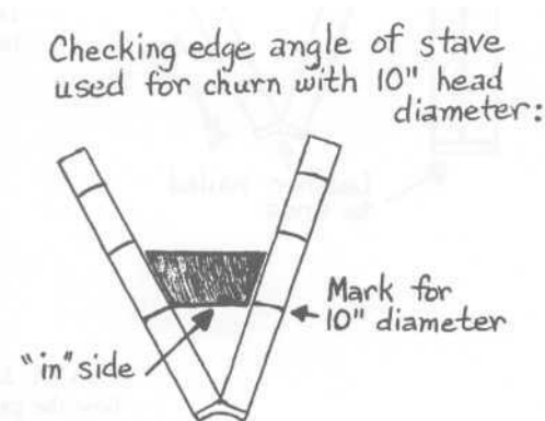
PLATE 341 The angled edges must fit the gauge as illustrated. The "in" side of the stave is the side placed on the mark.
