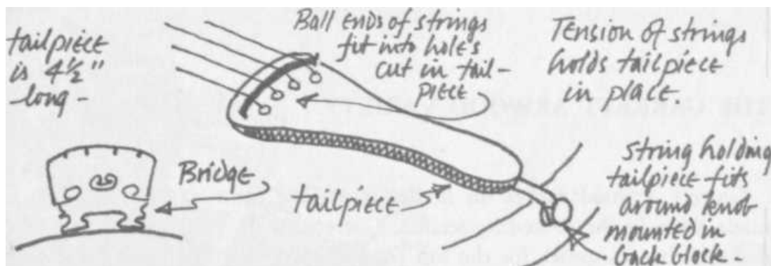
PLATE 122 Diagram of tailpiece and bridge.
