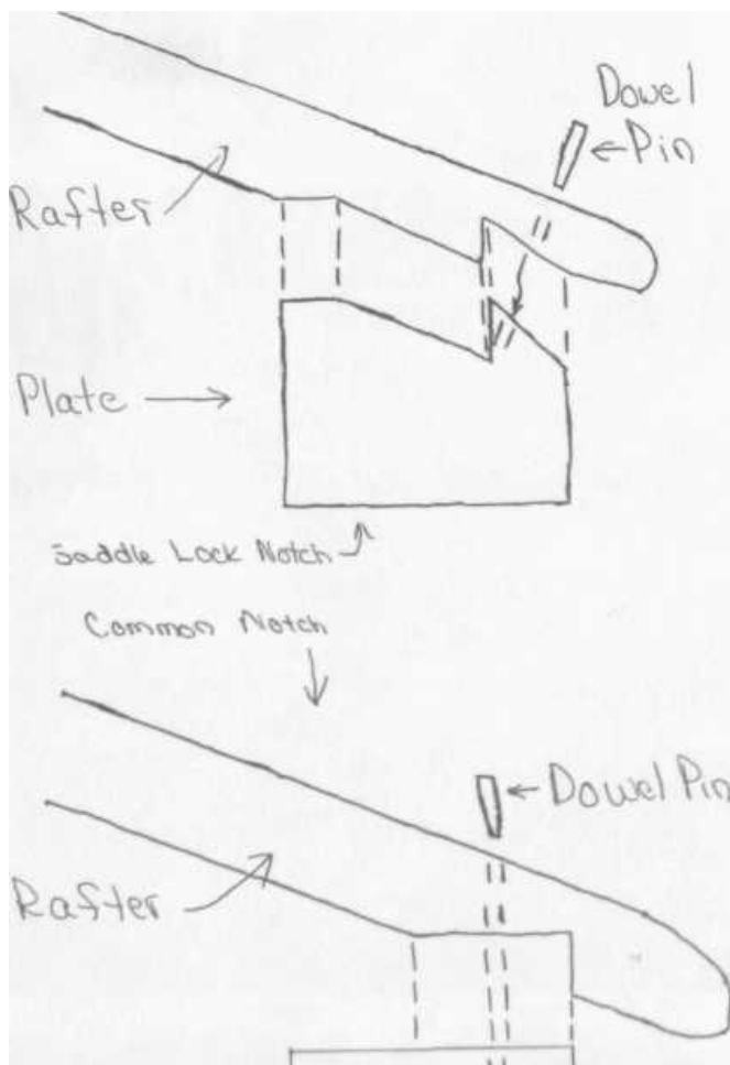
PLATE 411 Two methods of pinning rafters to plates.
