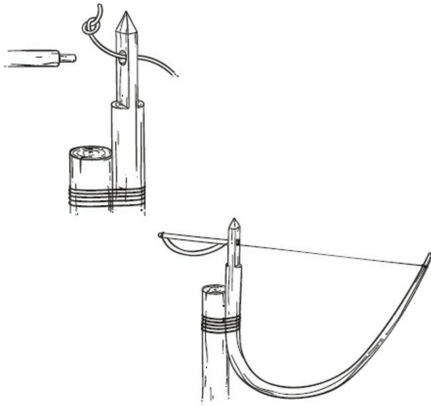
Ojibwa trap
