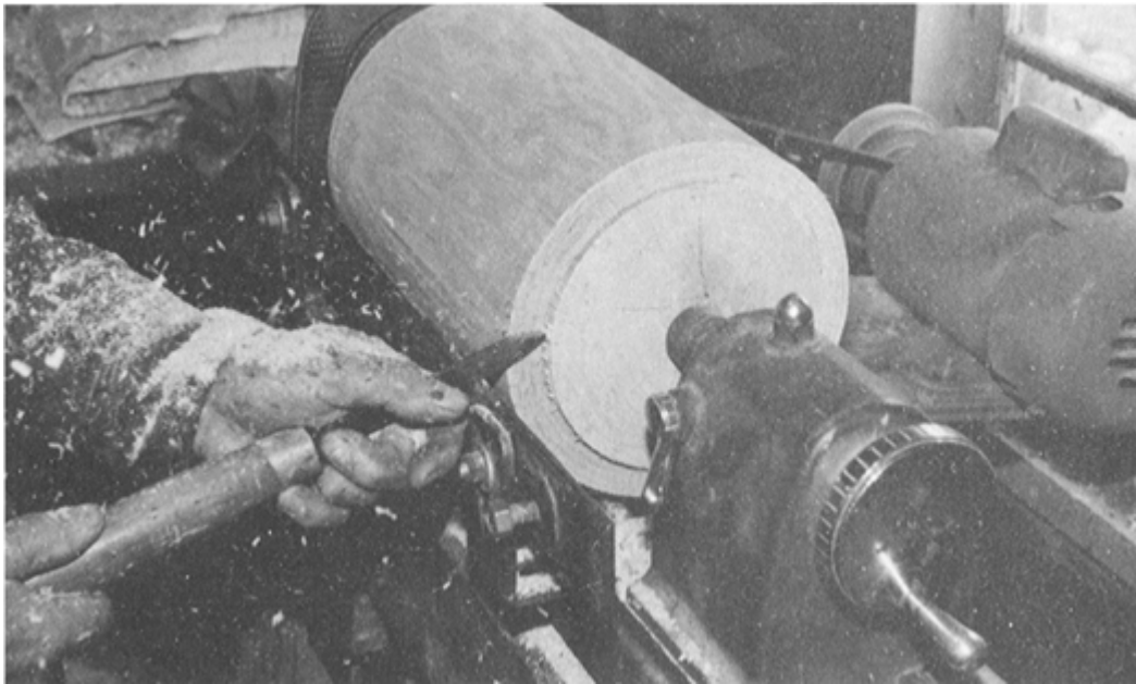
PLATE 197 Because it is nearly impossible to cut off the ends of each block exactly square with a band saw, Jud now uses a cutoff tool to square up the ends.
