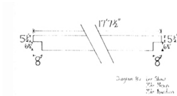
PLATE 409 The measurements for the floor joists for the first floor of the two-story section.
