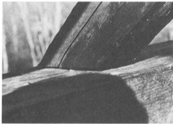
PLATE 418 With the final 48-foot-long wall logs anchored into place, the original rafters were replaced and pegged at their bases into the wall logs.
