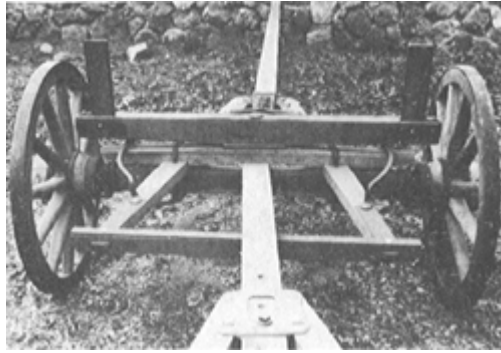
PLATE 321 The finished front assembly as seen from the rear.
