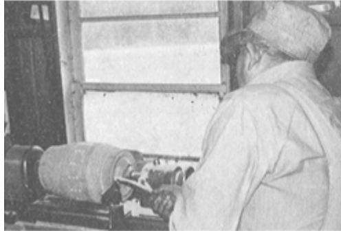
PLATE 204 After the holes are drilled, he puts the hub back in the lathe to hollow out the end that goes next to the wagon in order to seat the bearing.
