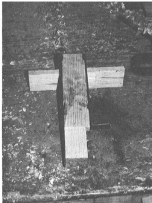
PLATE 312 ... and shapes the base of each into a tenon to fit the mortises in the bolster.
