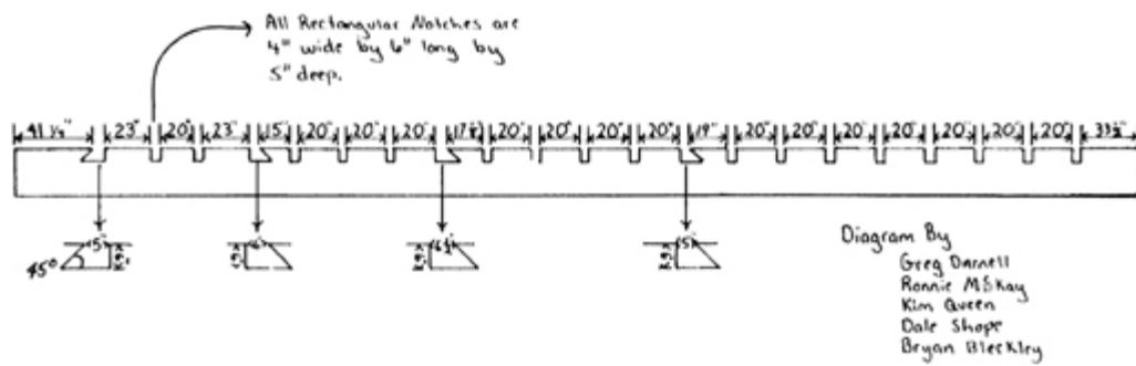
PLATE 410 One of the sill logs for the F-G addition.
