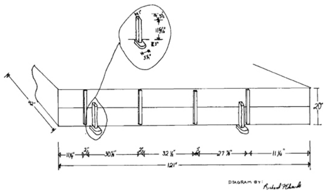
PLATE 337 Dimensions of the wagon bed.
