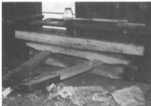
PLATE 300 Then he sets the bolster in place with the pin to double-check his progress. Note that a metal plate corresponding to the plate on the sand board has been bolted to the bottom of the bolster, and mortises have been cut in the ends of the bolster for the stakes that will hold the wagon bed in place.
