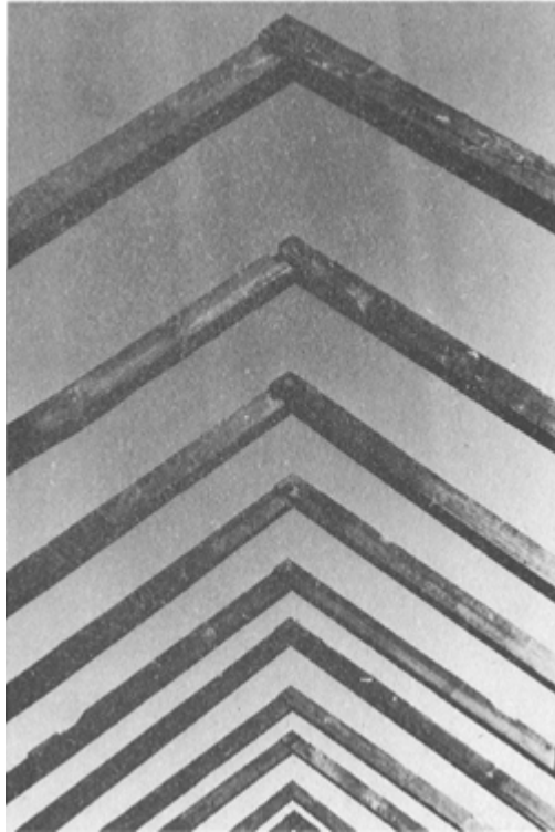
PLATE 420 Their lap-jointed peaks were also repegged together.
