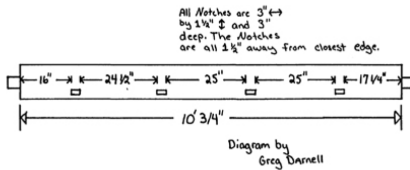
PLATE 427 The top of the long sill was also mortised at regular intervals to hold the vertical wall studs.
