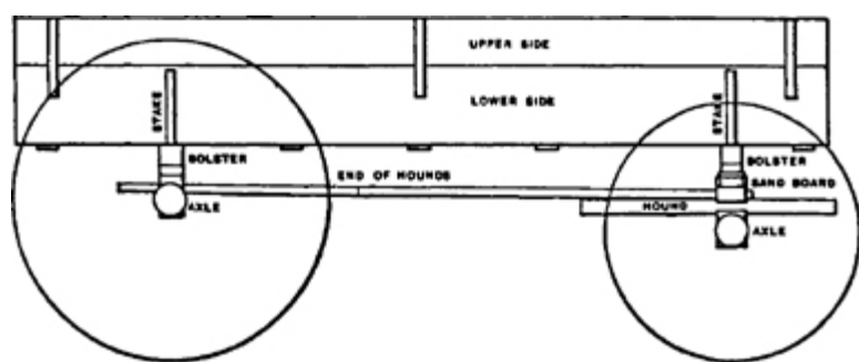
PLATE 338 Side elevation. (From PCB).
