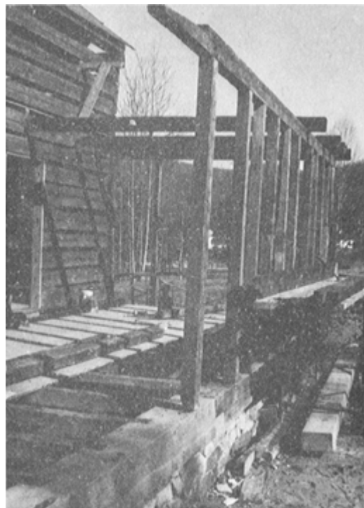
PLATE 439 This plate, the one that follows, and the accompanying diagram show how the two sections of the stringer that runs the length of the addition were shaped and joined and pegged in the middle.
