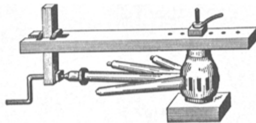
PLATE 234 With the cone as a guide for the hollow auger or spoke auger, he can now shape the ends of the spokes into the round tenons that will go into the felloes (fellies). (Since the felloe end of the spoke is the weak end, the trick is to have as large a tenon as possible to hold the felloes on without breaking off, and yet small enough to leave a good bearing surface for the felloes. According to Practical Carriage Building , many makers leave half the width of the tenon—a fourth on each side—for shoulders.
