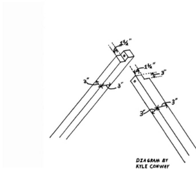
PLATE 420 Their lap-jointed peaks were also repegged together.
