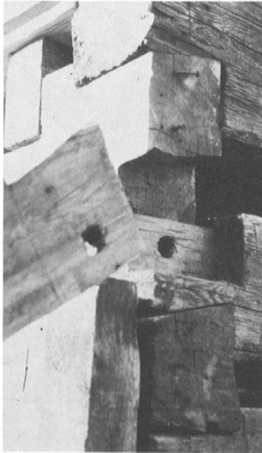
PLATE 442 The porch stringers at each end of the addition not only fitted down over the mortises cut into the vertical corner support posts, but their opposite ends were also notched and pegged into the wall of the main part of the house itself.
