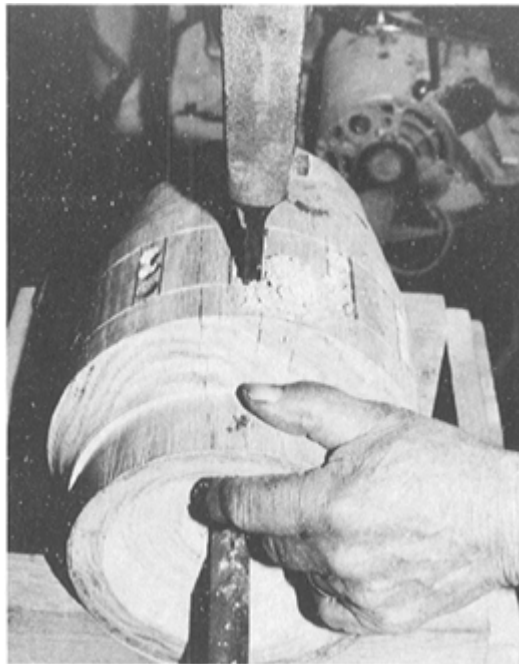
PLATE 207 With a mortising bit, he drills out each mortise to its size of five-eighths inch by two inches.
