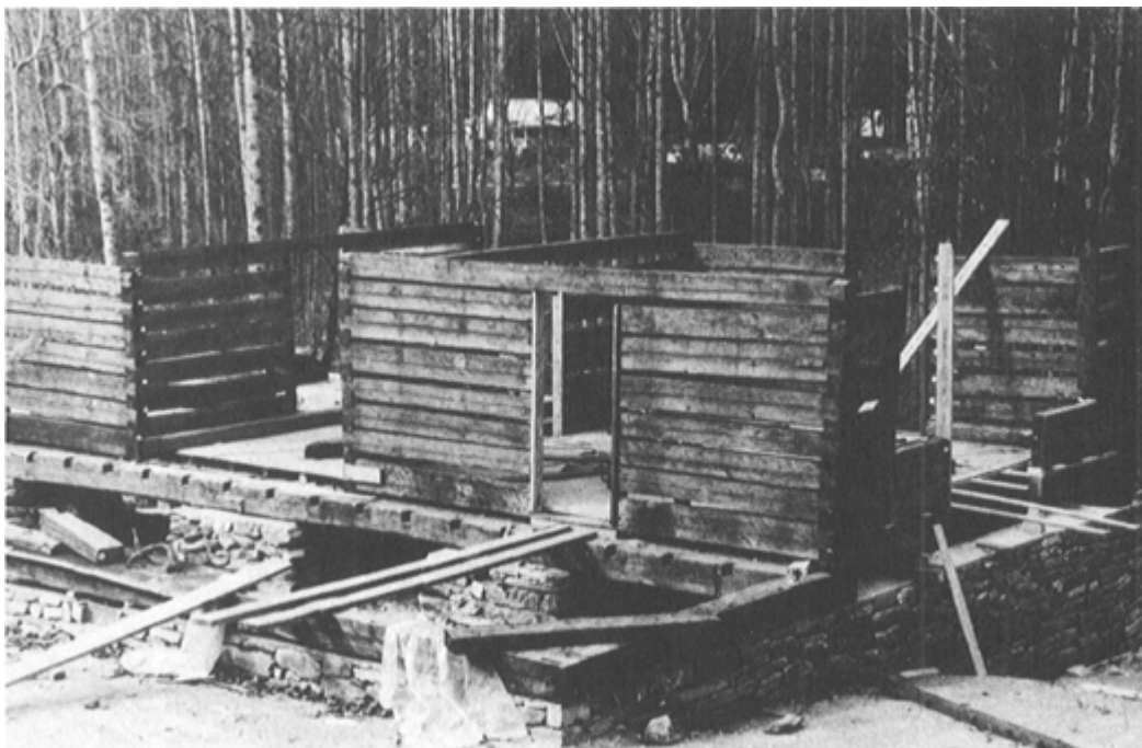
PLATE 415 Door jambs and window frames were repegged as in the original house.
