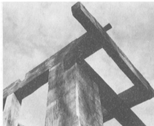
PLATE 399 When the kitchen was removed, an elaborate piece of mortised and pegged work was revealed, supporting the roof line for the dining room, F, at a point where F and H had joined around the kitchen chimney.
