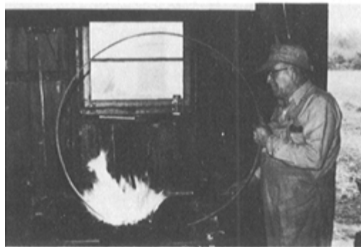
PLATE 253 ... heats the ends to a white heat, or approximately 2,400 degrees Fahrenheit ...
