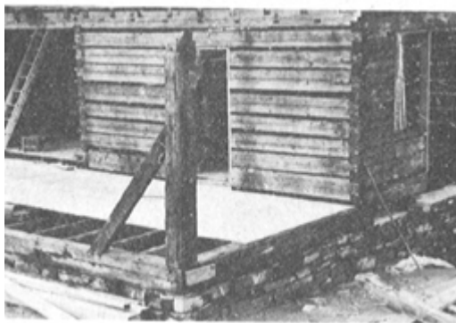
PLATE 428 The vertical corner post was fitted back into its mortise, and its diagonal brace was replaced and pegged.
