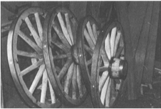
PLATE 266 Four finished wheels.
