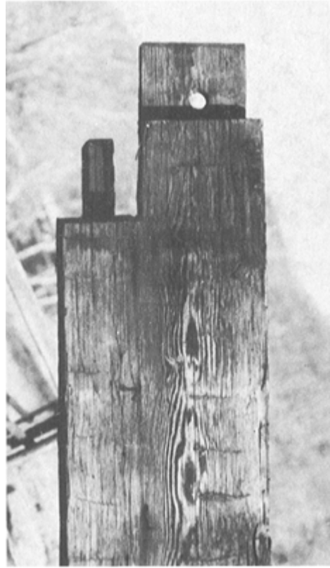
PLATE 433 The top of each vertical corner post was shaped into tenons to hold the porch stringers.
